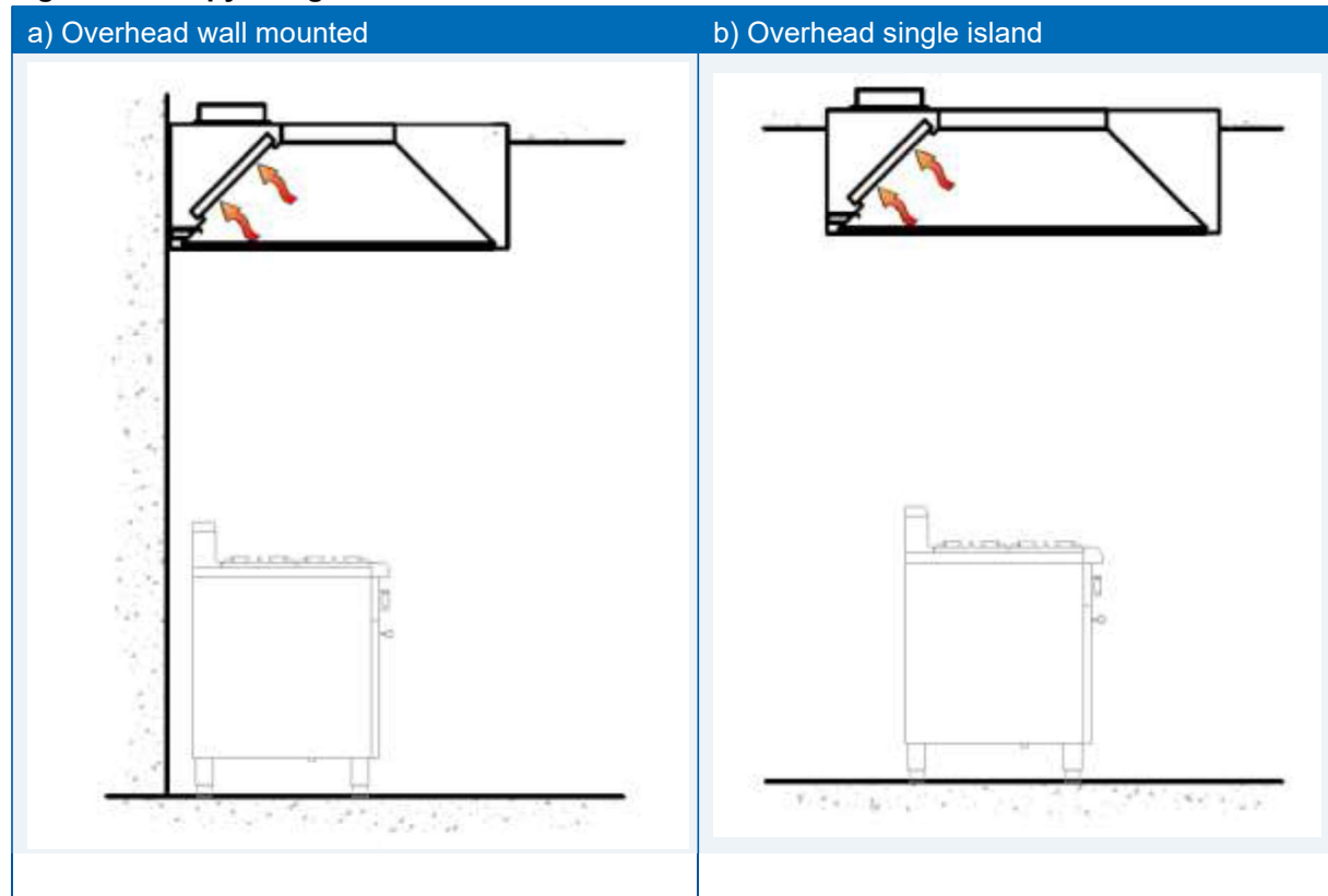
Figure 3: Canopy design
