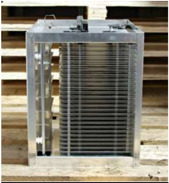
Electrostatic precipitator after cleaning
