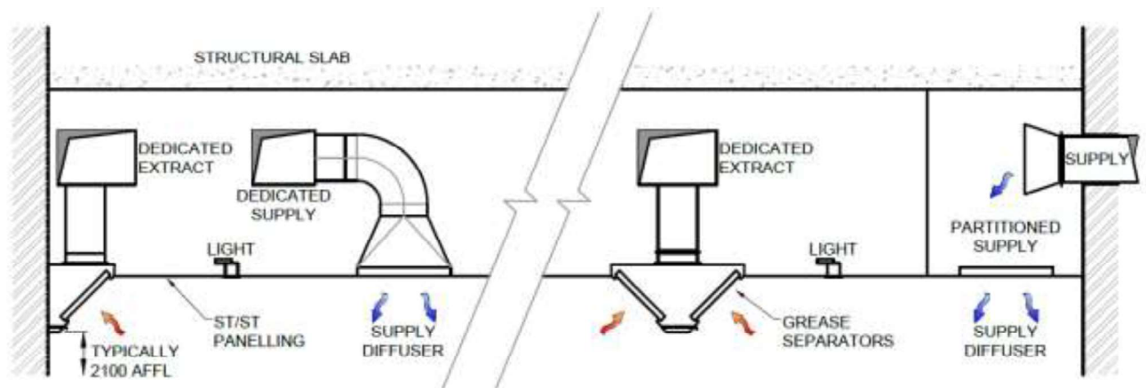
Figure 6 : plenum ceiling
